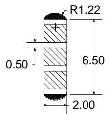
Column, Sectioned
